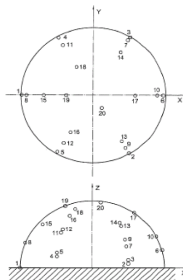
Figure 2: Microphone positions for MF720
